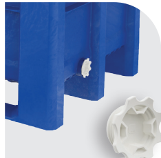
Integral drain port (long and short side) Dolav 56x4 BCS
