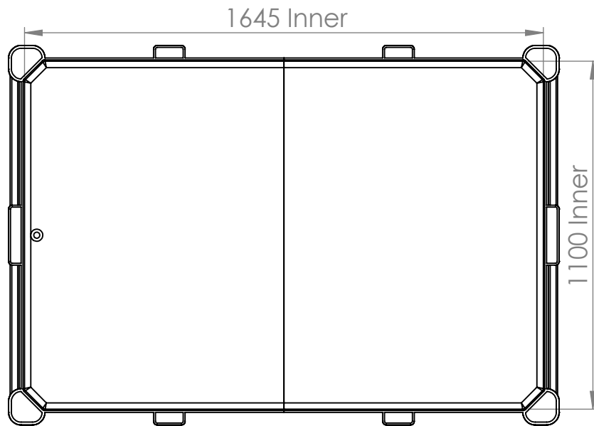
Top view (without base)
